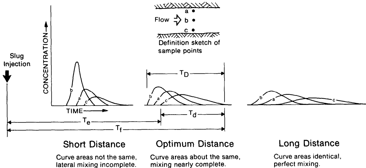
Figure 1.—Typical response curves observed laterally and at different distances downstream from a slug injection of a tracer in the center of a stream.
