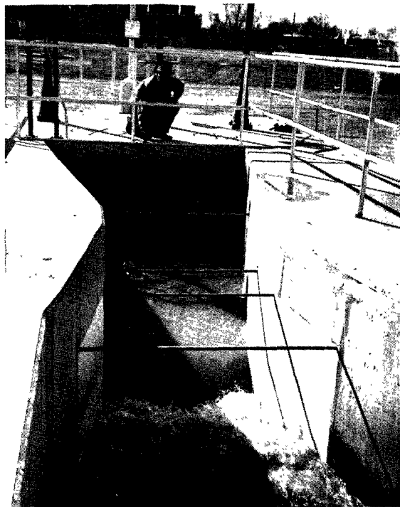
Figure 21.—Multiple dye injection in the approach to a Parshall flume; not visible is dye-injection pump, which preinjects dye into a hose line from a domestic water supply. Eight samples taken across the channel about 10 ft below the hydraulic jump in the bottom of the picture yielded good results.
