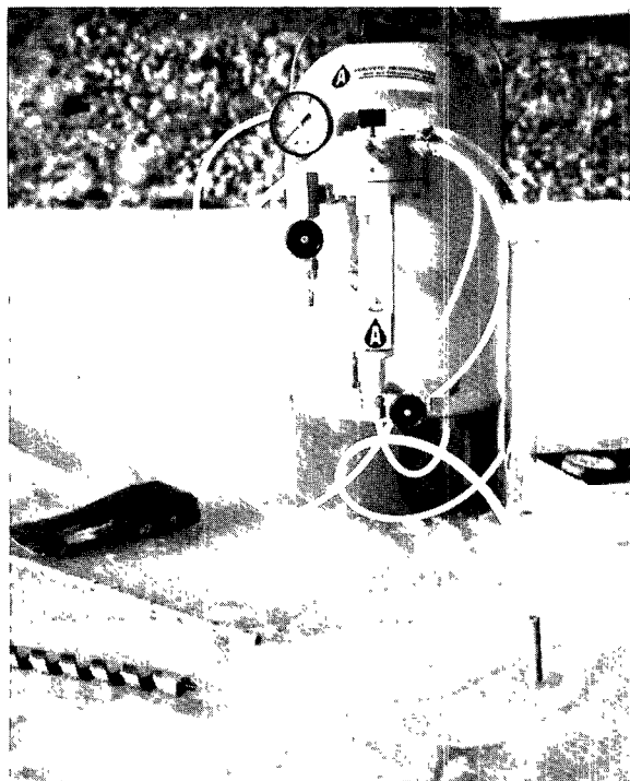
Figure 25.—Dye injection under ice cover, using a chemical-feed tank. An auger is used to drill holes through the ice and a tube is used to draw background samples from under the ice before injection.
