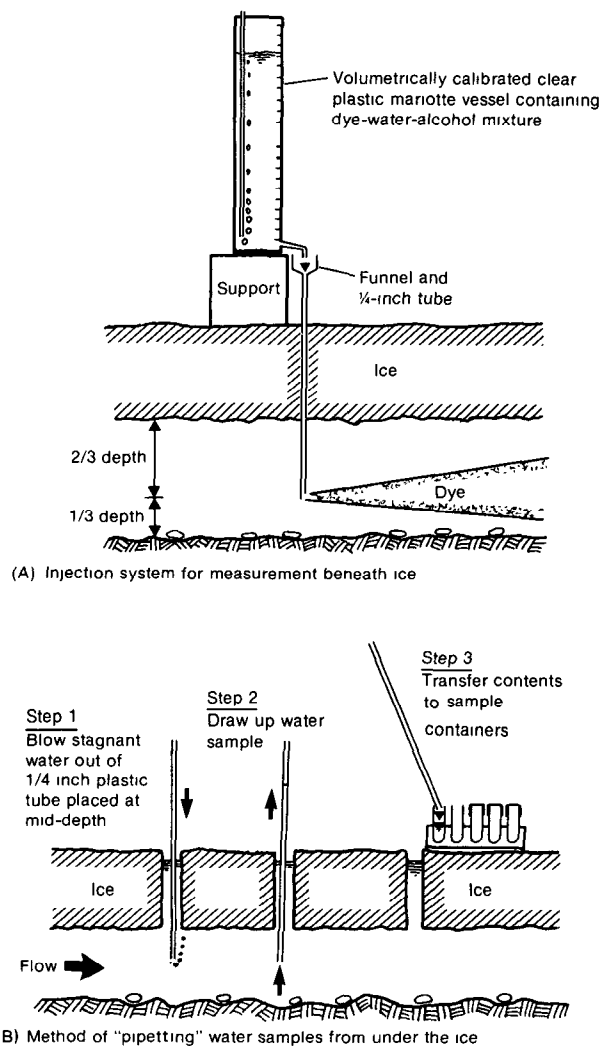
Figure 24.—Dye-dilution discharge measurement under ice cover.
