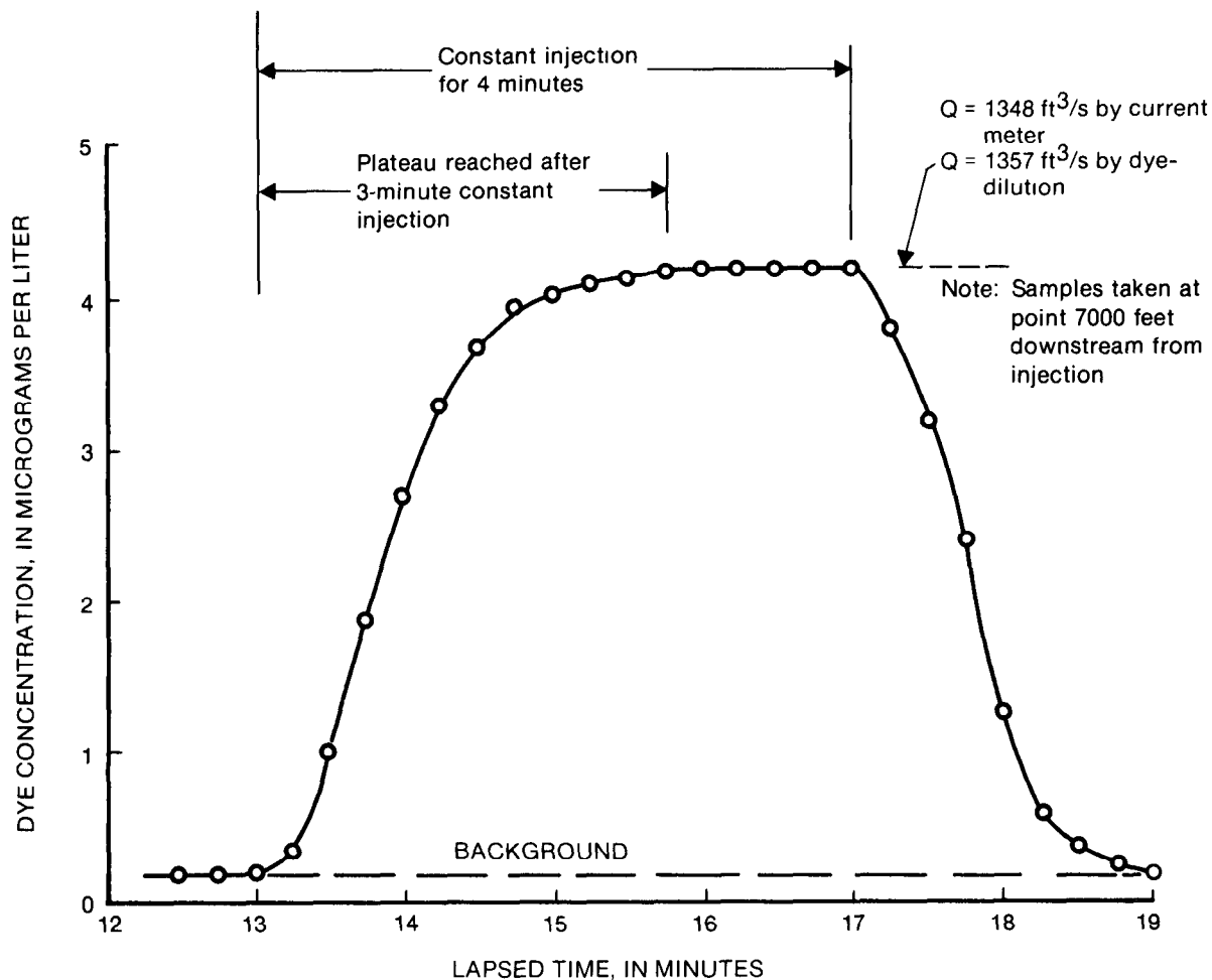
Figure 28.—Rapid measurement of discharge in a lined canal by dye dilution, Charles Hanson Canal, Colorado.
