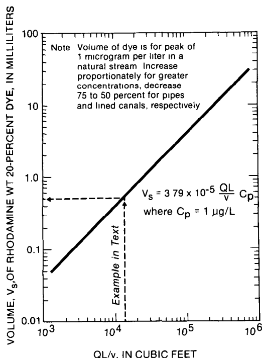
Figure 4.—Quantity of rhodamine WT 20-percent dye required for slug injection to produce a peak concentration of 1 microgram per liter at a distance downstream, L , at a mean velocity, v , and with a discharge, Q , in the reach.
