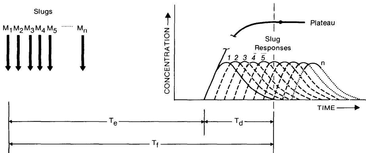
Figure 2.—Superposition of slug-response curves to simulate constant-injection buildup to a plateau at one location in a stream section.
