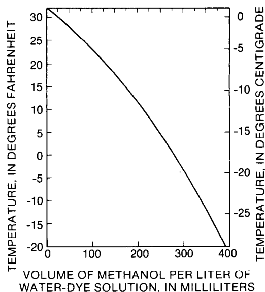
Figure 27.—Proportions of methanol alcohol and water-dye solution needed to prevent freezing of mixtures at selected temperatures.
