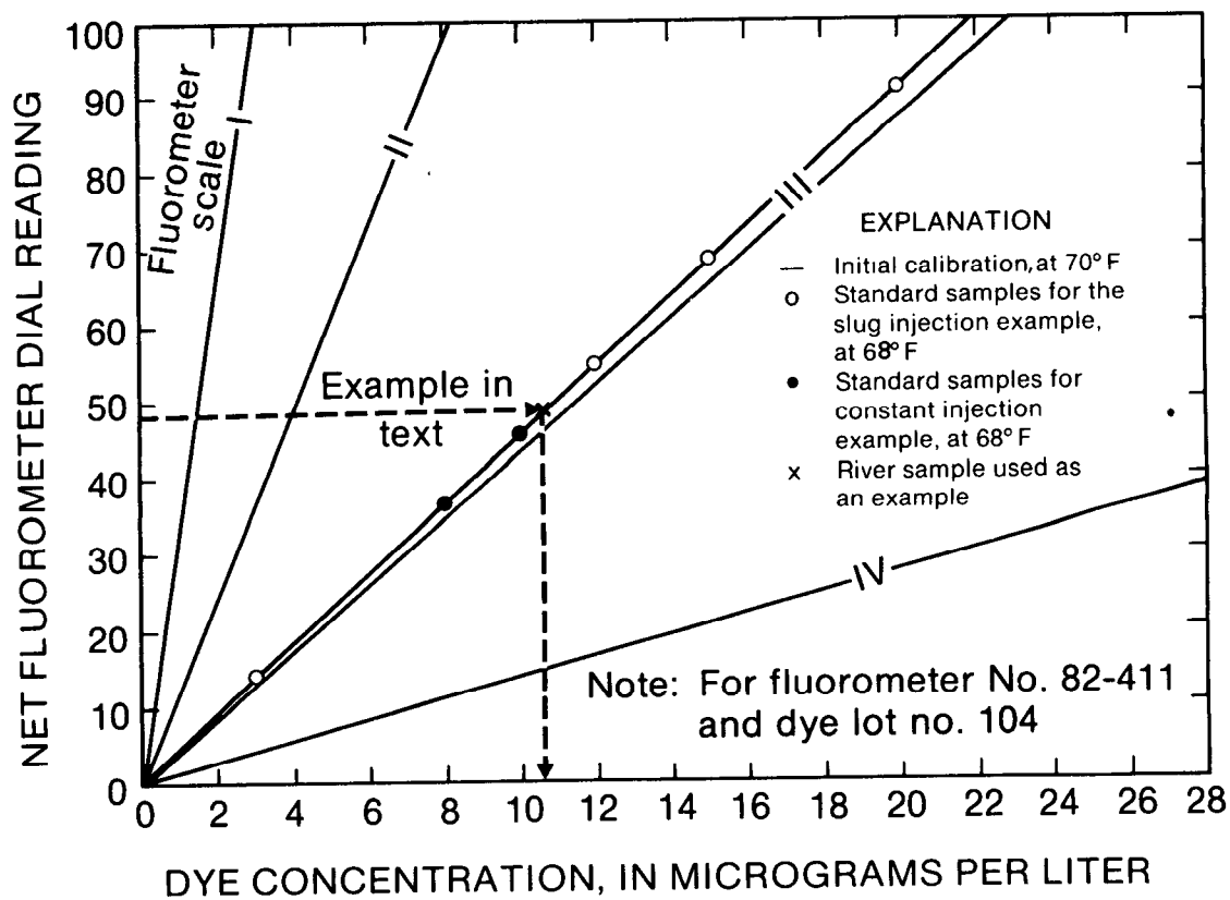
Figure 7.—Typical calibration curves for a fluorometer.
